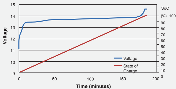
Charge Voltage &amp; State of Charge (SoC) @ 0.33C charge rate
